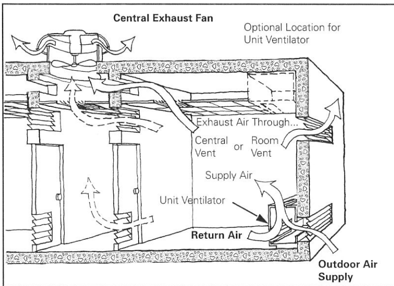
Air Supply through a Unit Ventilator
